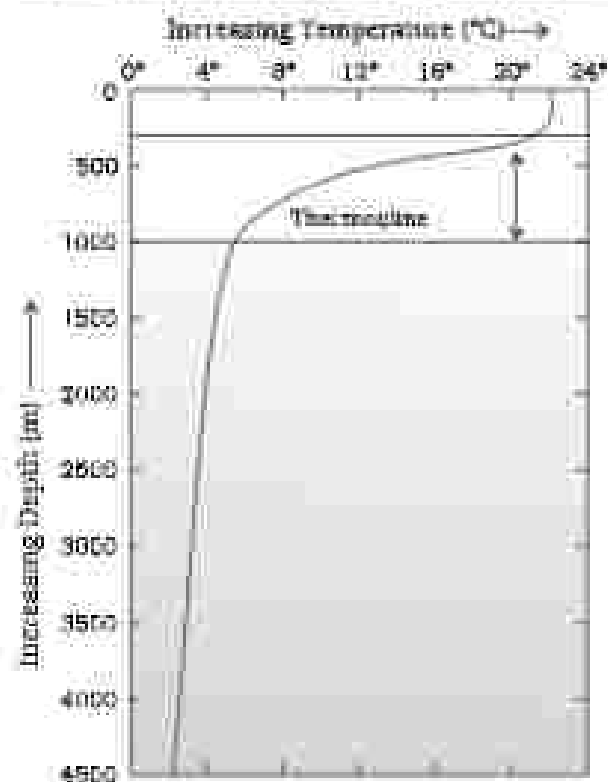
Figure 13.3 : Thermocline
