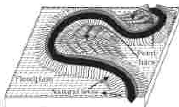
Figure 7.6 : Natural levee and point bar
