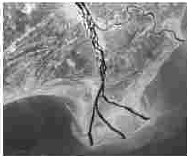
Figure 7.5 : Aerial view of part of Krishna river delta, Andhra Pradesh
