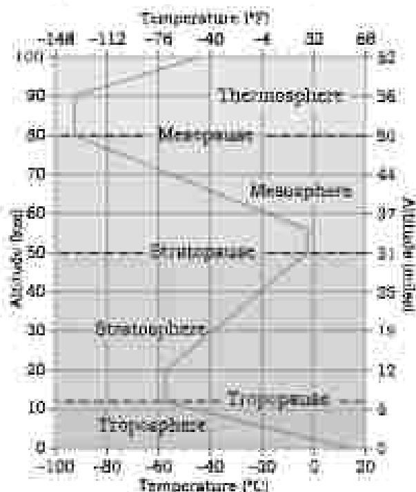
Figure 5.1: Structure of atmosphere
