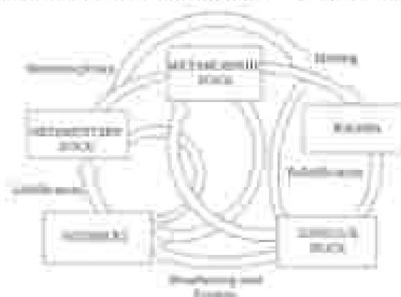
Fig 5.1 / Rock Cycle
