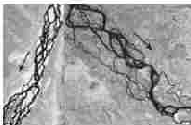
Figure 7.9: Satellite scenes showing braided channel segments of Gandak (left) and Son (right) rivers. Arrows show the direction of flow
