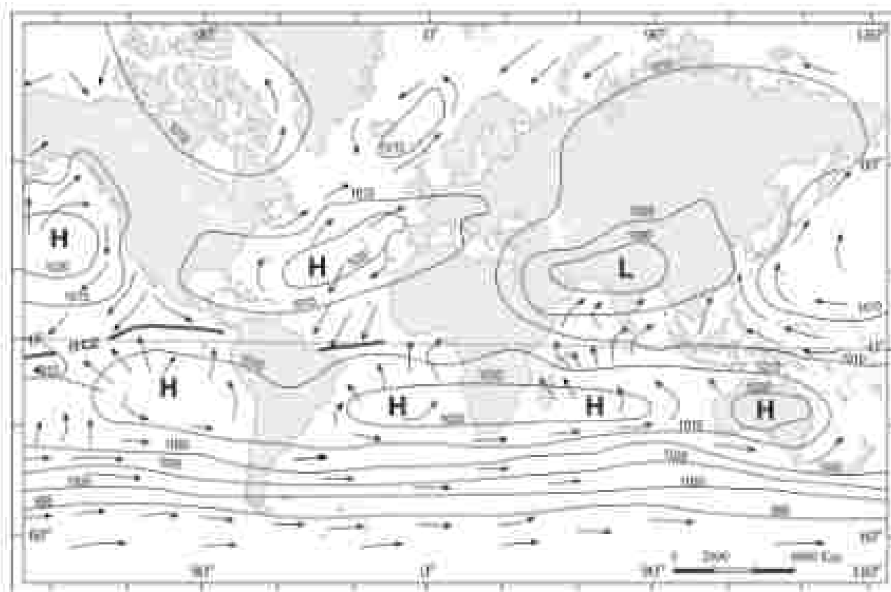
Figure 10.2 : Distribution of pressure (in millibars) — July
