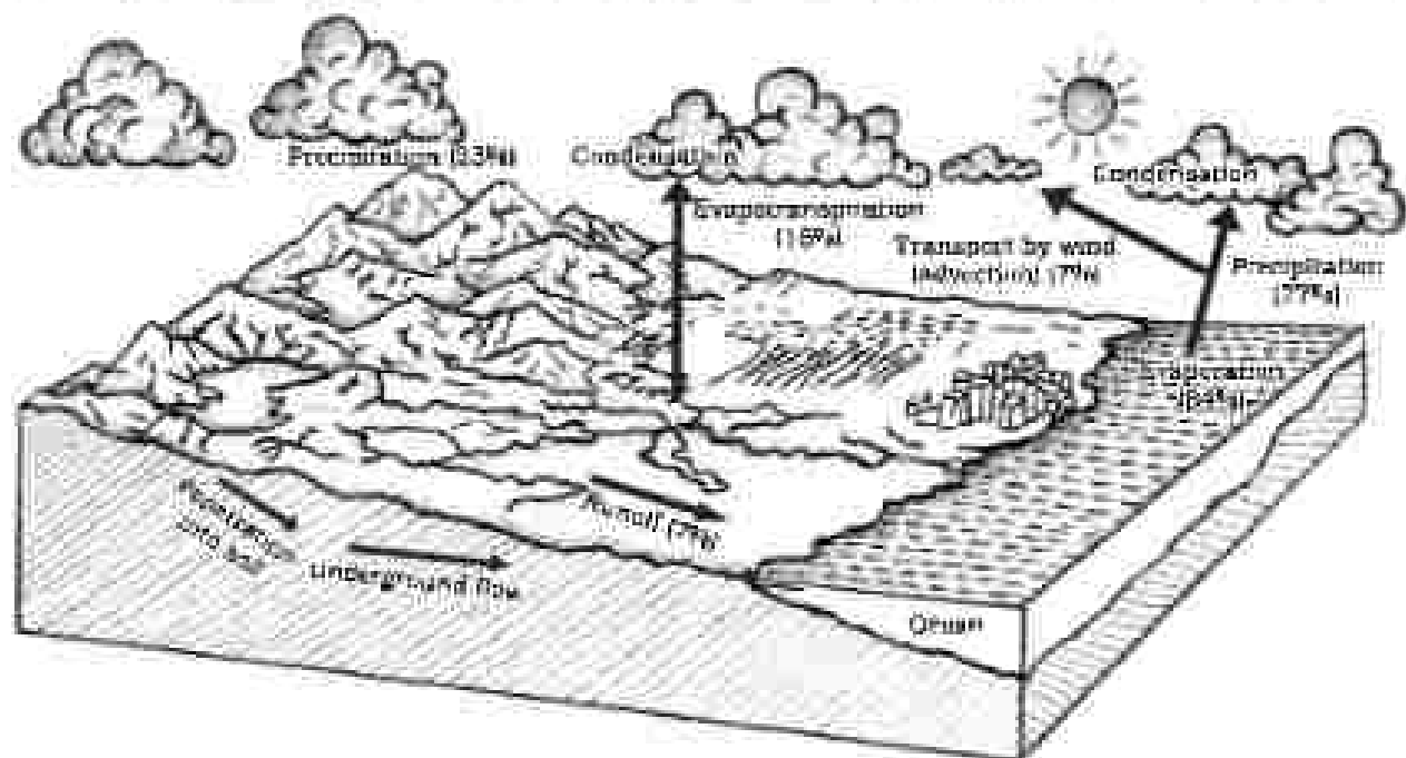
Figure 13.1: Hydrological Cycle
