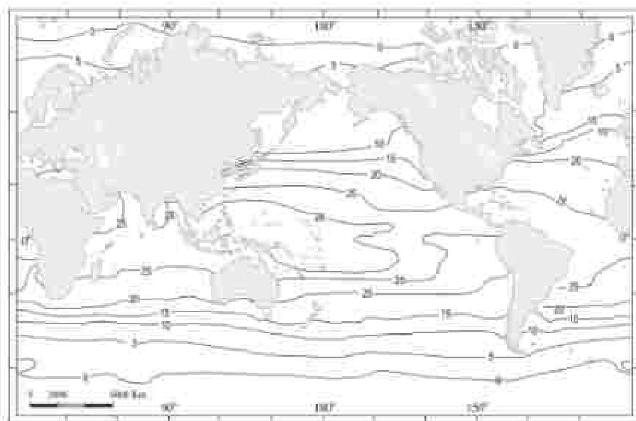
Figure 13.4 : Spatial pattern of surface temperature ( ^{\circ}\text{C} ) of the ocean
