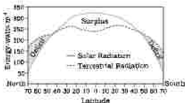
Figure 9.3 : Latitudinal variation in net radiation balance
