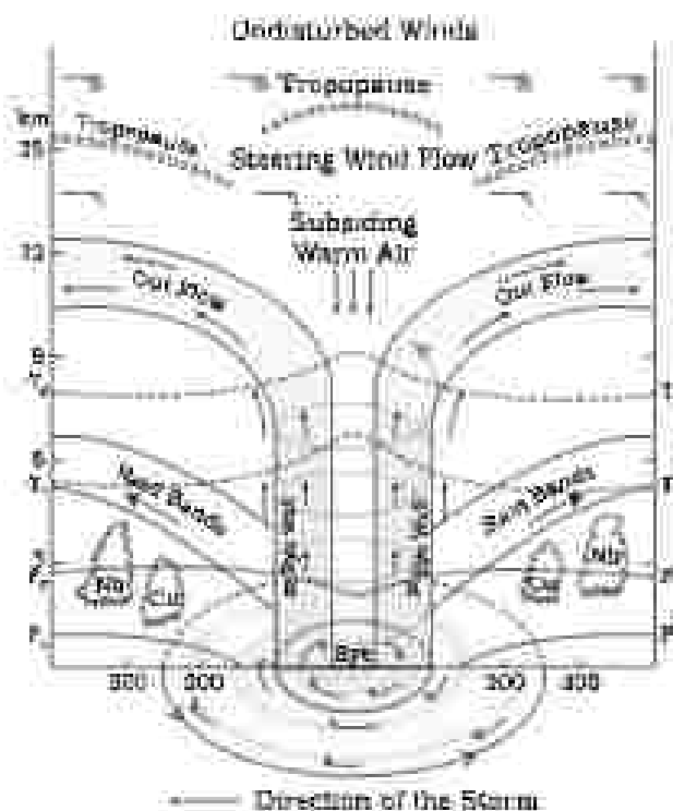
Figure 10.10 : Vertical section of the tropical cyclone (after Rama Sastri)
