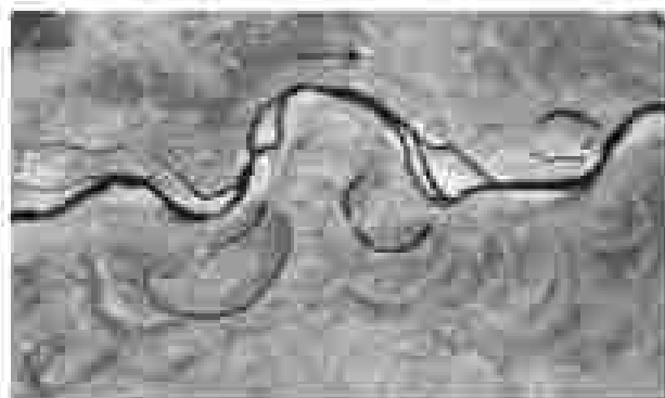
Figure 7.7 : A satellite scene showing meandering Rapti-Gandak river near Munaffapur, Bihar, showing a number of oxbow lakes and cut-offs
