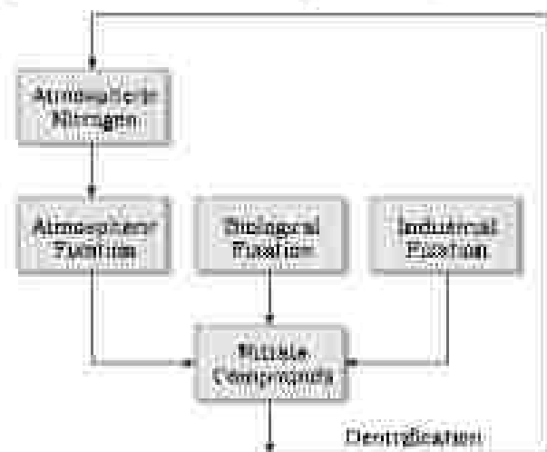
Figure 15.3 : Nitrogen Cycle
