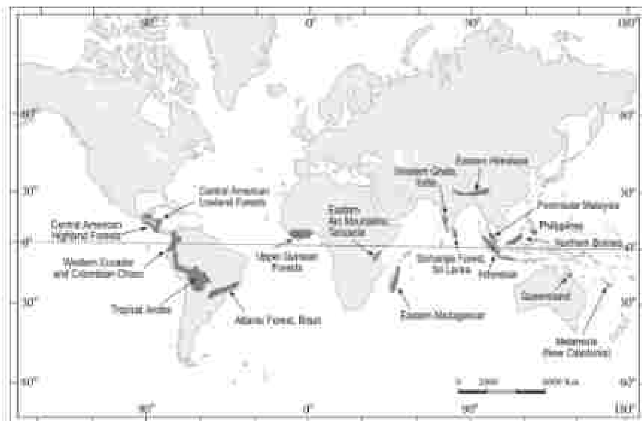
Figure 10.5: Ecological 'hotspots' in the world.
