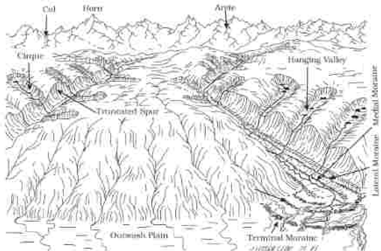
Figure 7.13: Some glacial erosional and depositional forms (adapted and modified from Spencer, 1982)
