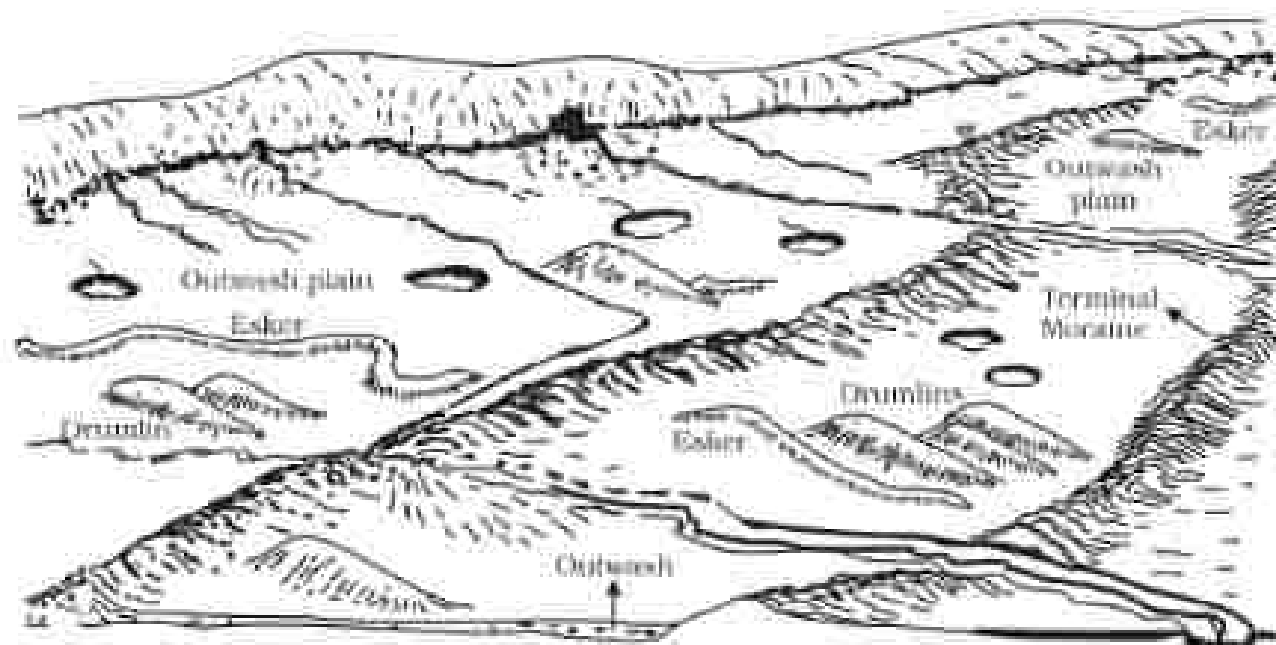
Figure 7.14: A panoramic diagram of glacial landscape with various depositional landforms (adapted and modified from Spencer, 1982)
