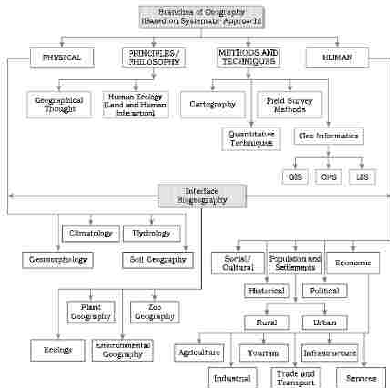
Figure 1.3 : Branches of geography based on systematic approach
