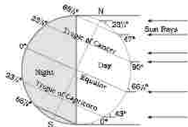
Figure 9.1 : Summer Solstice
