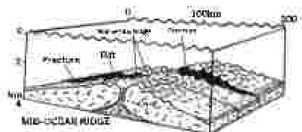
Figure 19.2 : Relief features of ocean floors
