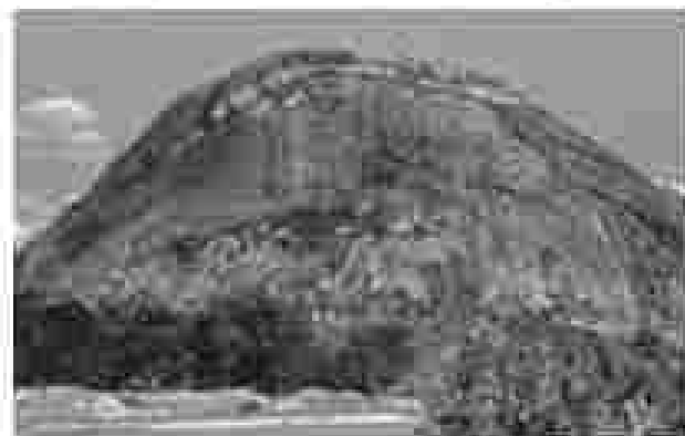
Figure 6.3: A large exfoliation dome in granite rock near Bhongir (Bhuvanagiri) seen in Andhra Pradesh.
